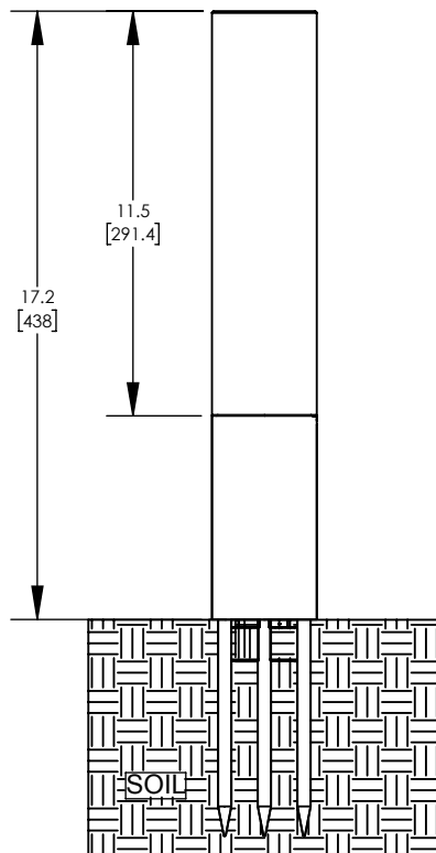
GM-3 - 3 Prong Stake Mount
